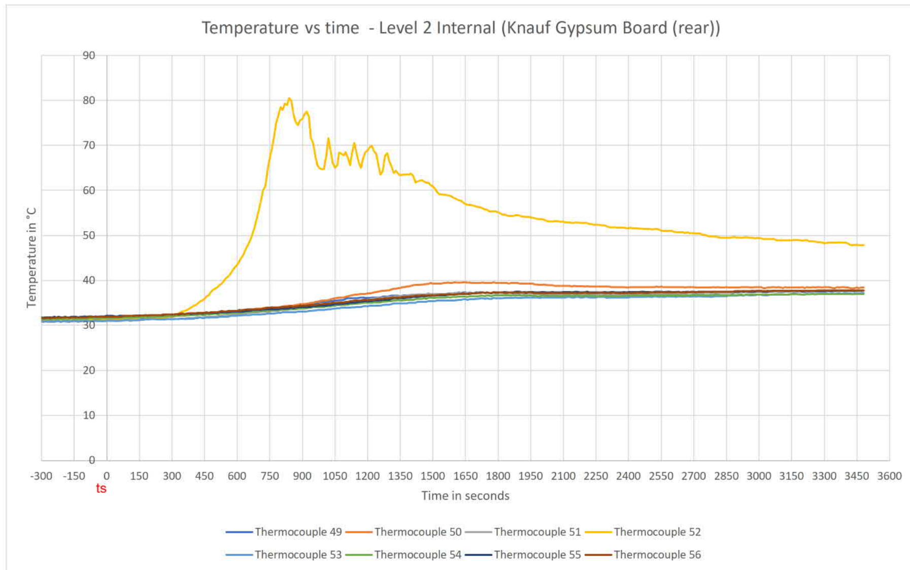
Figure 11 Level 2, internal, Knauf gypsum board (rear) – temperature vs time
